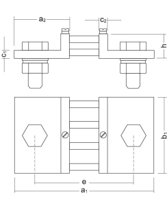
SHUNT 200-1000
