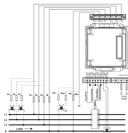
Measurement system: 4W-3 Ph (MC3 type transformer (.../0.250A))
